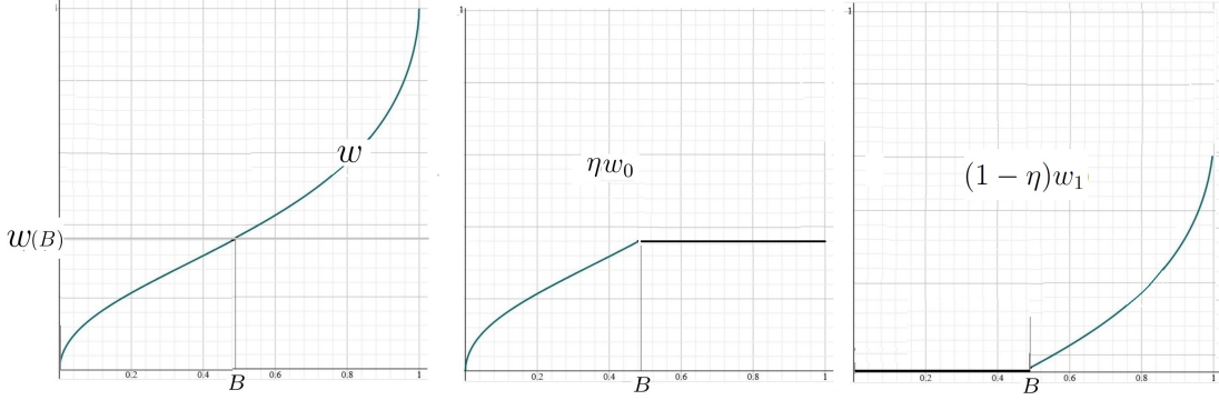
Figure 1: Decomposition of the inverse S -shaped distortion function w of (29) with parameter r = 0.61 and inflection point B \approx 0.48 .
